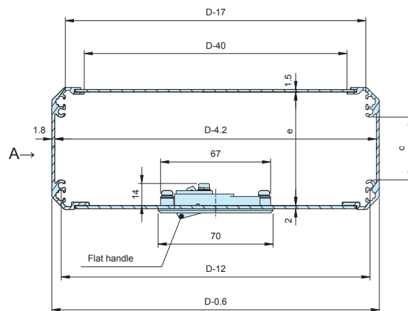
D cross-section
