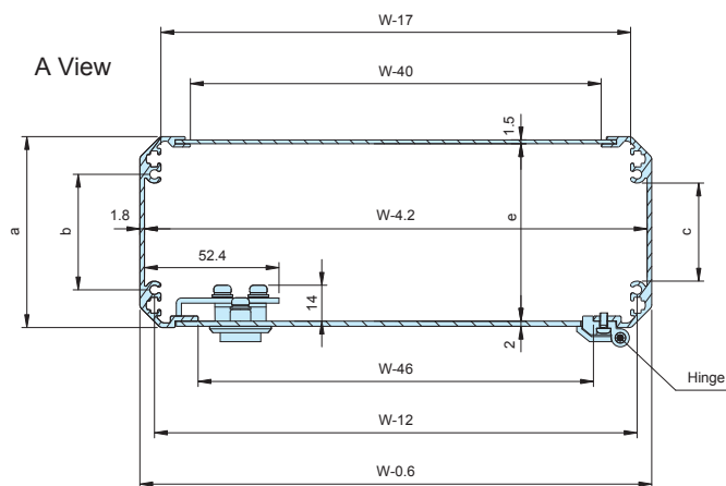
W Cross-section
