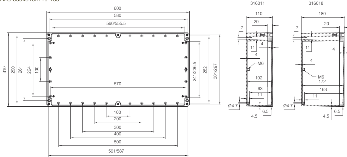
ALU 600x310x110-180
